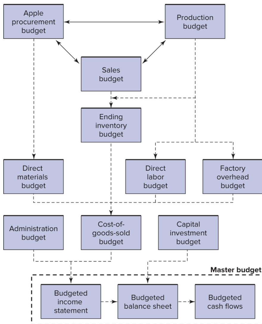
Figure 1: Logical flow
